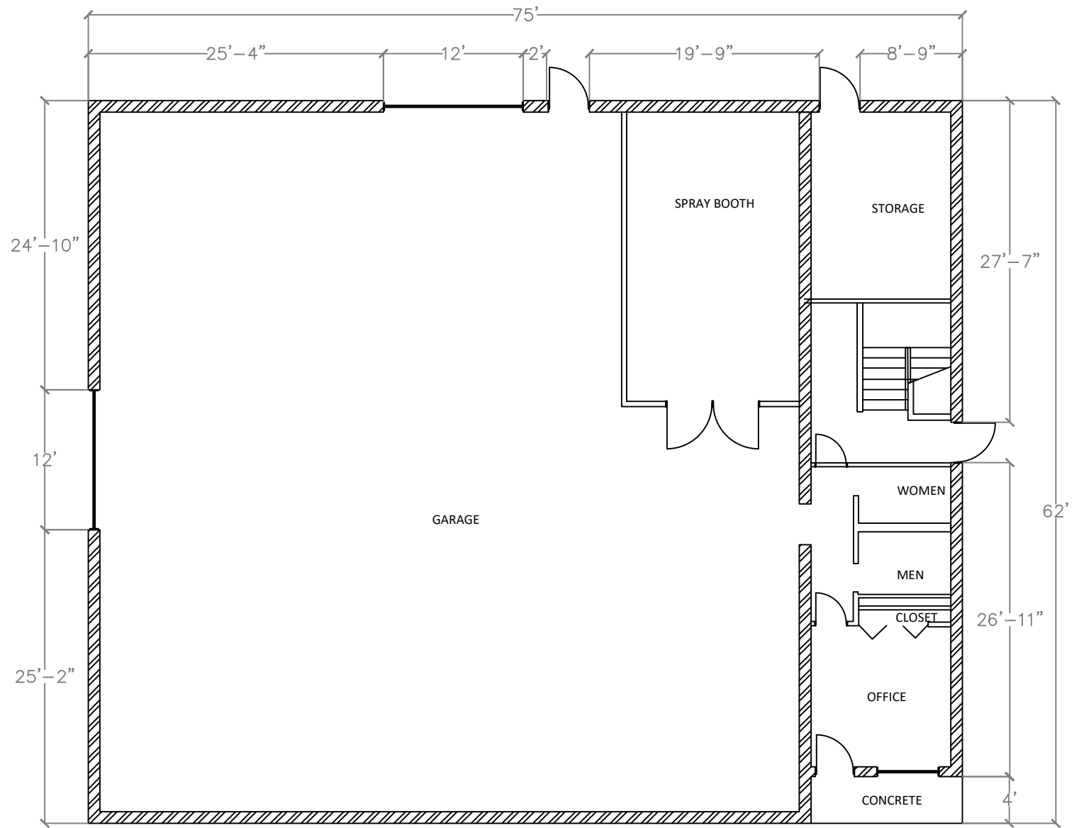
214 LEDYARD STREET FLOOR PLAN 4,600SF
