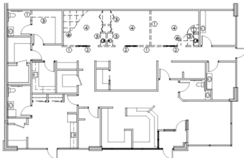
1. DEMO PLAN SCALE: 3/16" = 1'-0"
