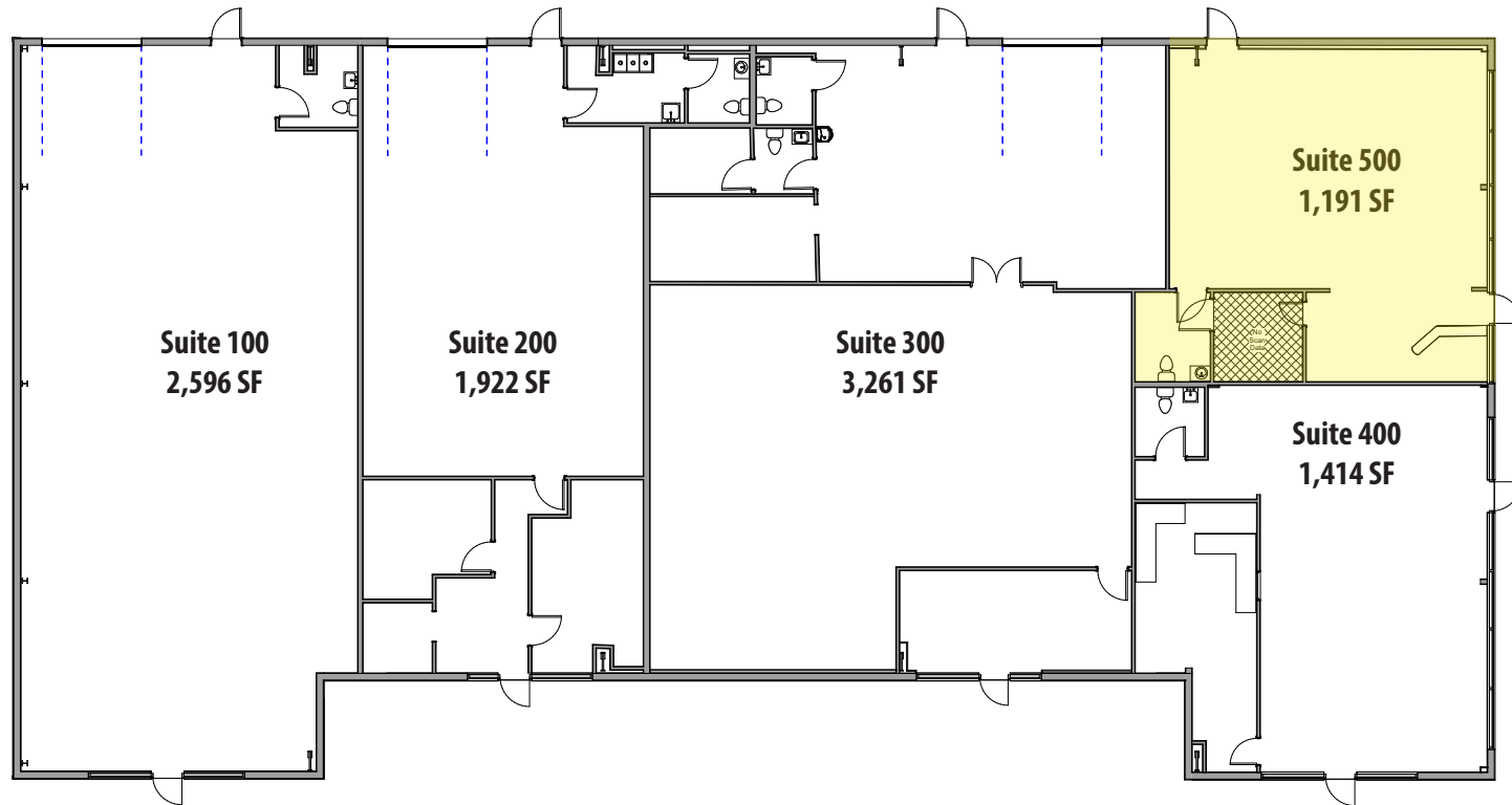
○ First Floor Plan 3/16" = 1'-0"
