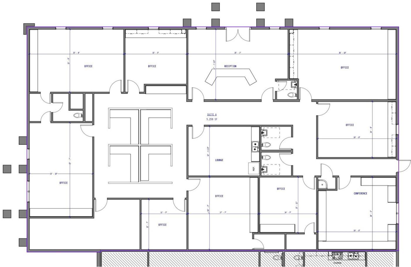
1 LEASABLE AREA PLAN 1/4" = 1'-0"
