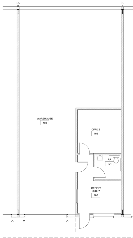
02 BUILD OUT - OPT. 2 1/4"=1'-0" @ 24 x 36 OFFICE BUILD OUT: 400 SF
