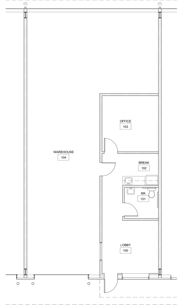
03 BUILD OUT - OPT. 3 1/4"=1'-0" @ 24 x 36 OFFICE BUILD OUT: 550 SF
