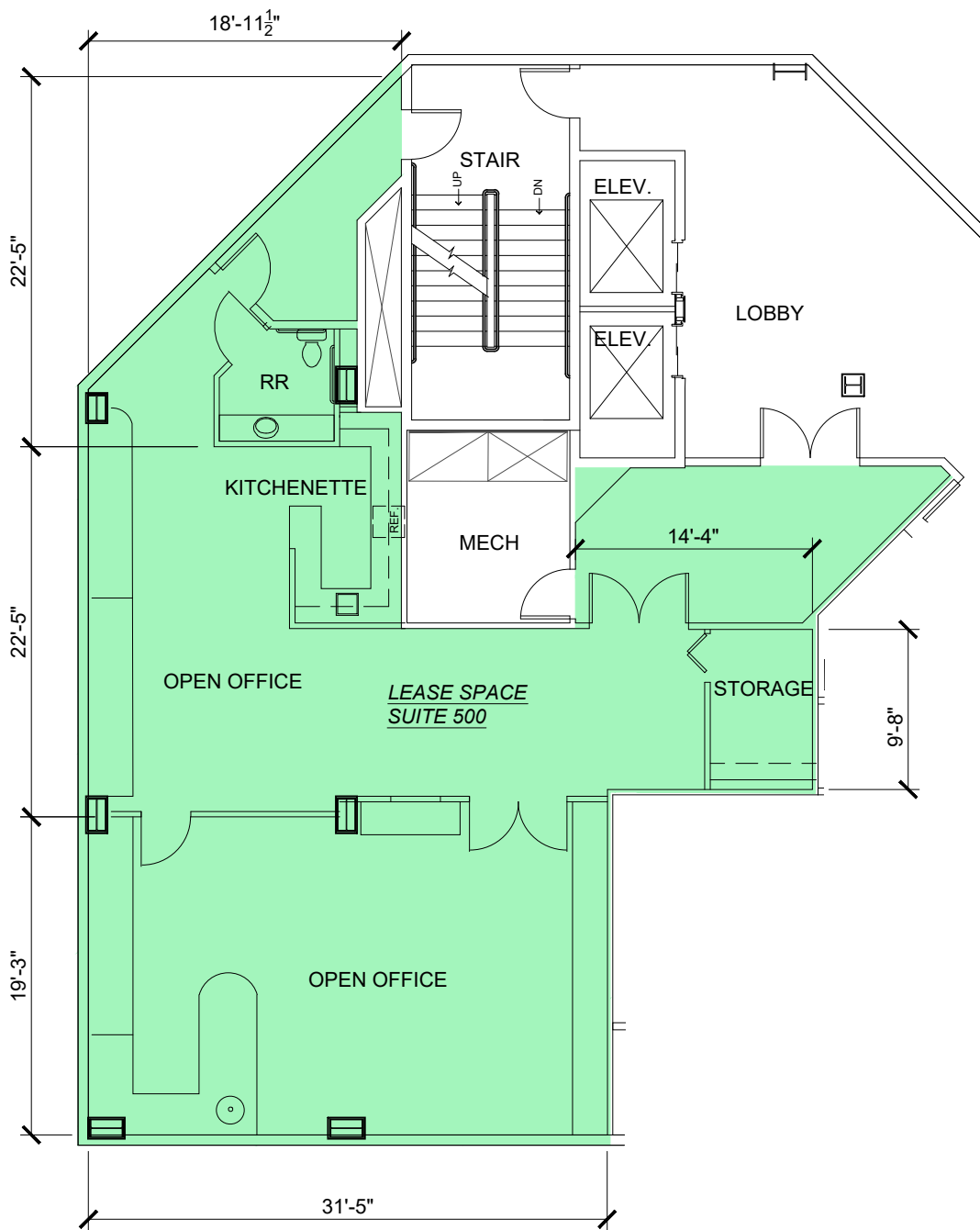
5th Floor Suite 500 Floor Plan Scale: 3/32" = 1'-0" 04/14/21
