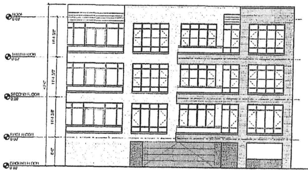
WEST ELEVATION
