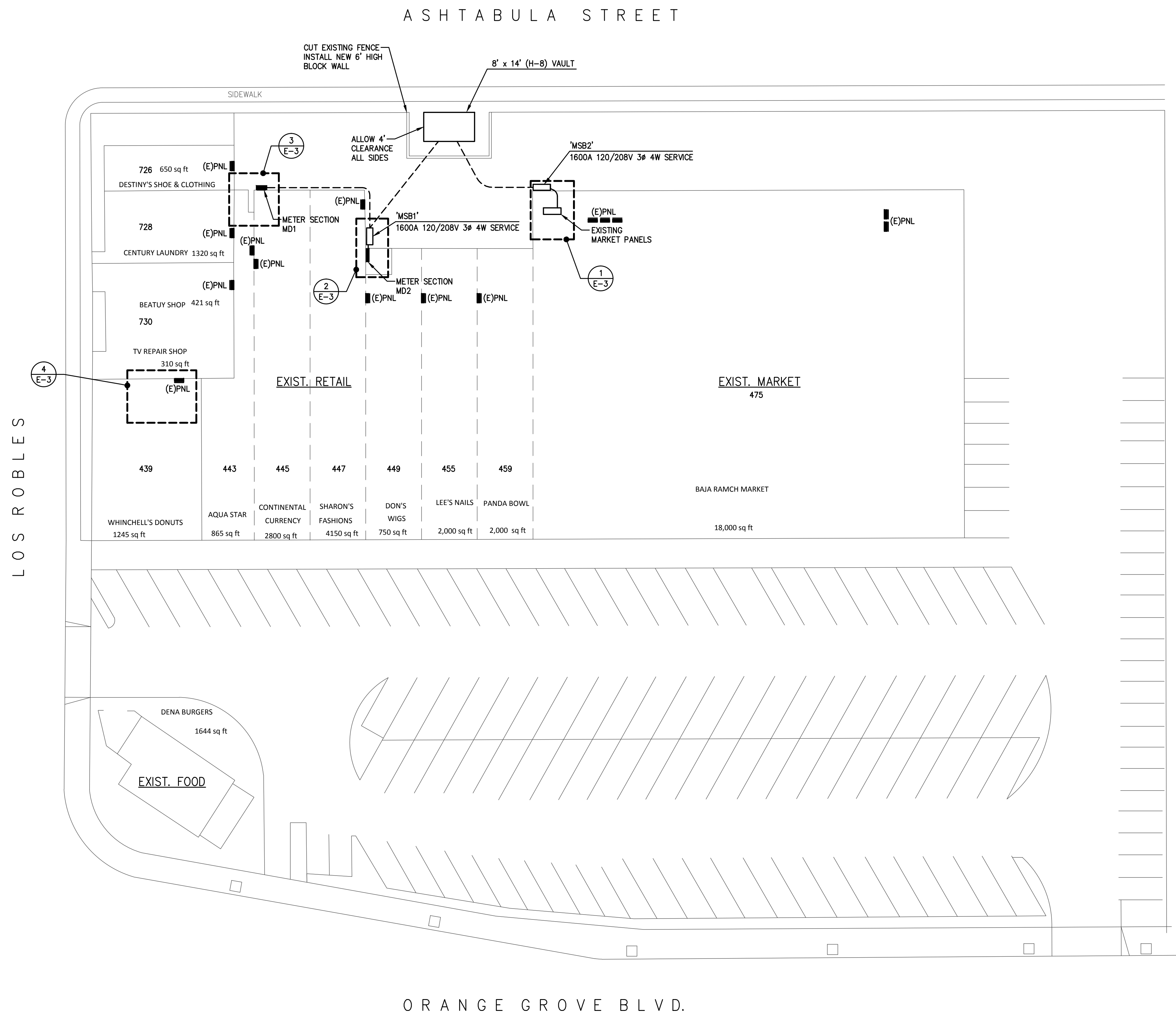
ELECTRICAL SITE PLAN SCALE 1/16"=1'-0" 1
