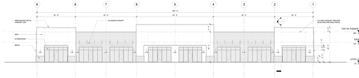
1 NORTH ELEVATION 1/8" = 1'-0"
