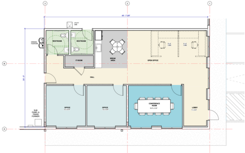
1 A-201 ENLARGED OFFICE FLOOR PLAN 1/4" = 1'-0"
