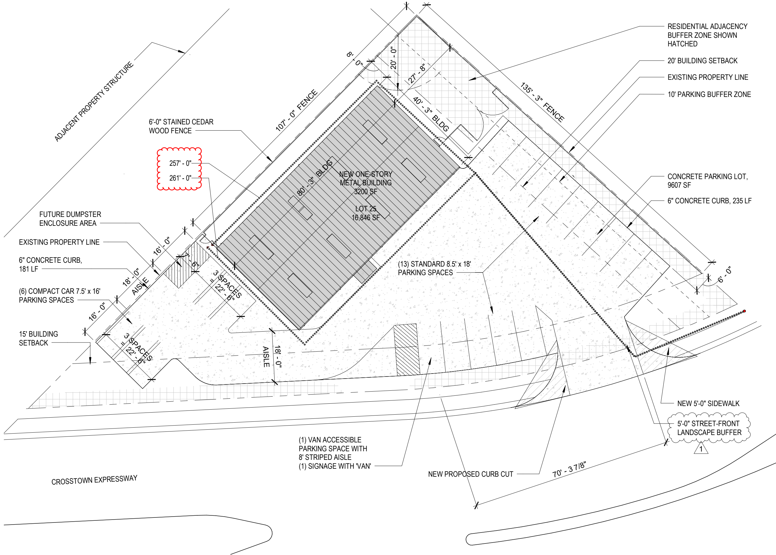
1 SITE PLAN 1" = 20'-0"
