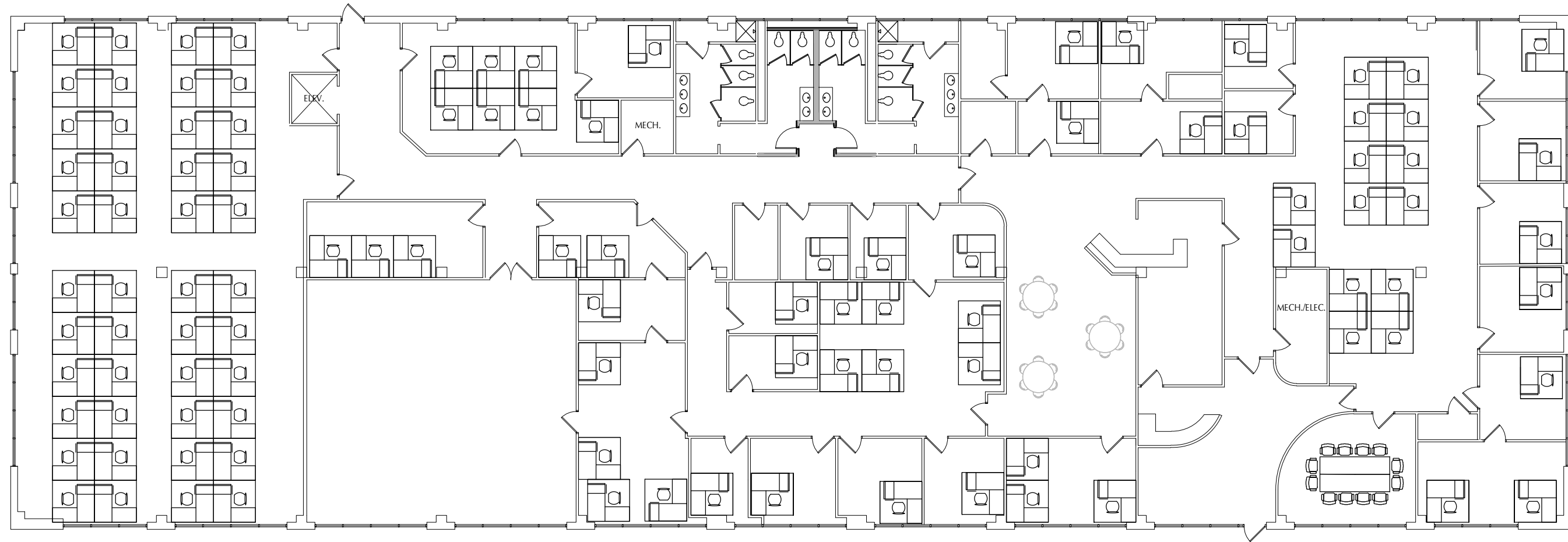
1 THIRD FLOOR PLAN A3.1 SCALE: 1/16" = 1'-0"
