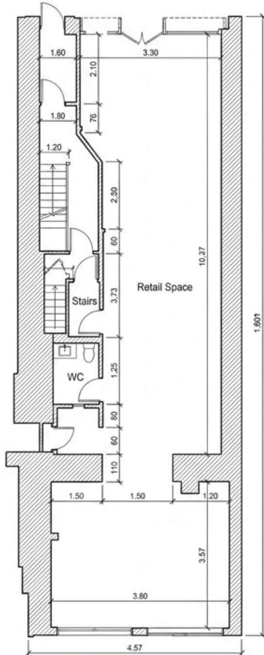
GROUND FLOOR - 1,677 SF (approx)
