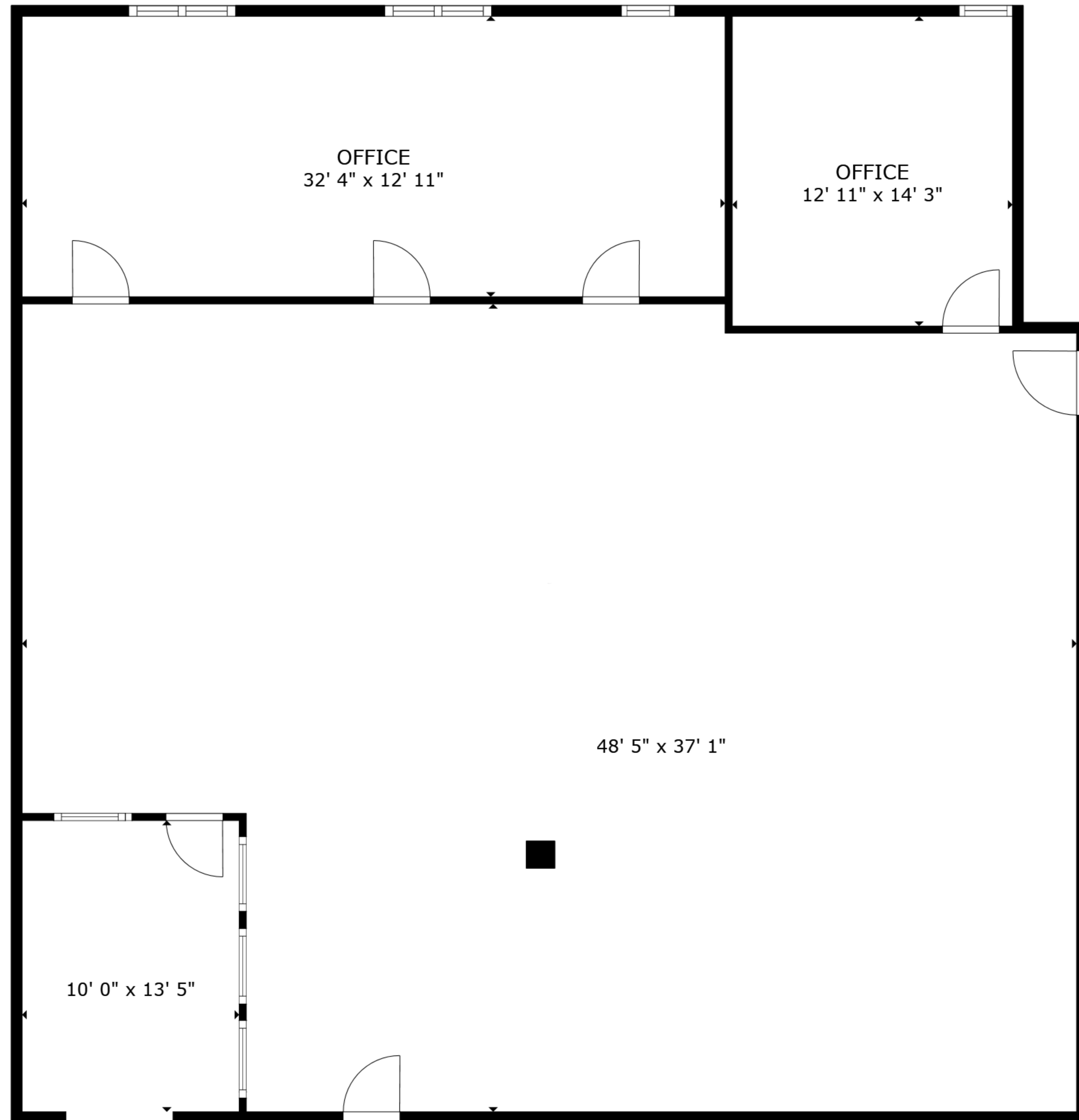
FLOOR PLAN
