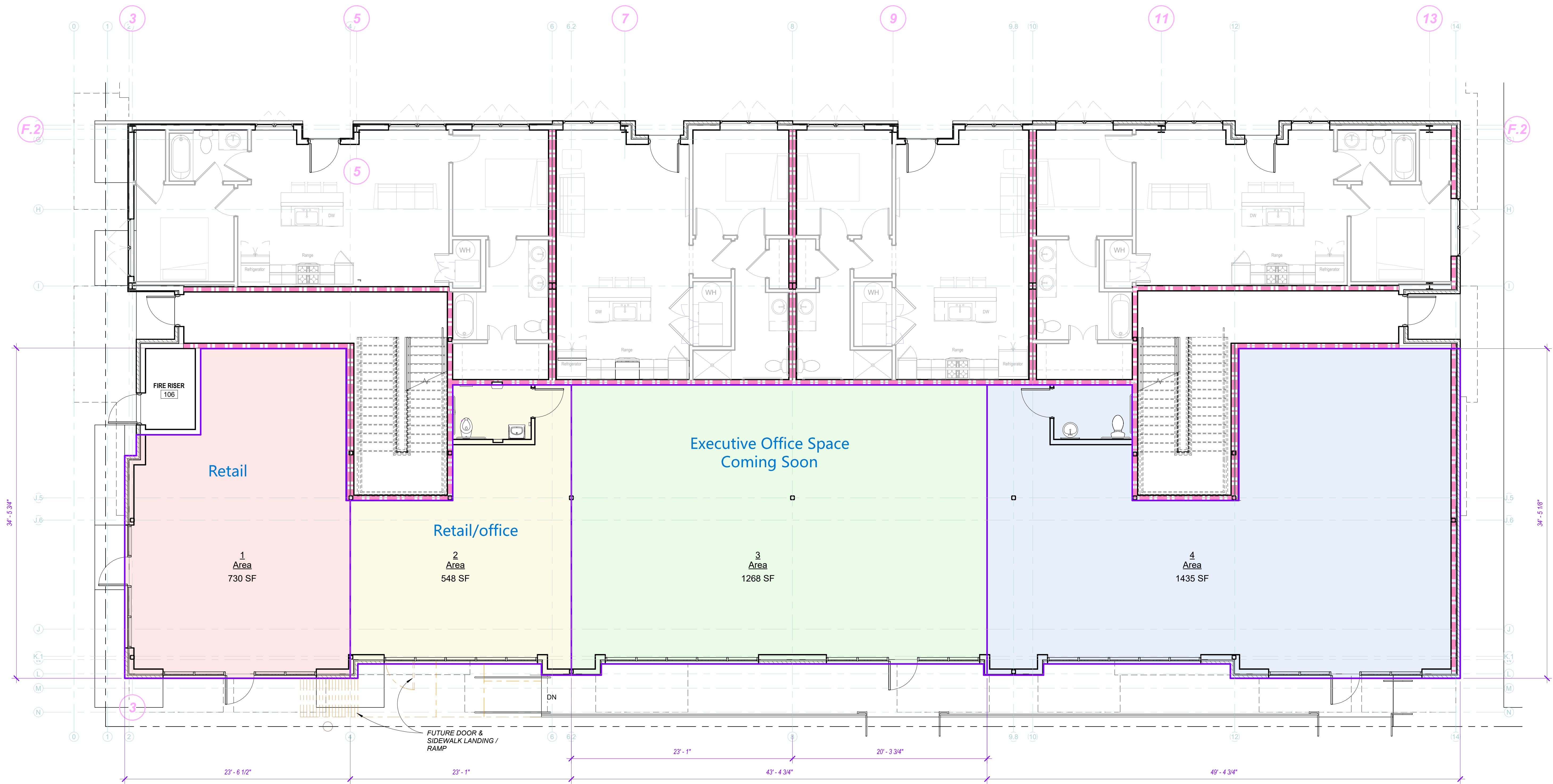
1 1st Floor Tenant Area Plan 3/16" = 1'-0"
