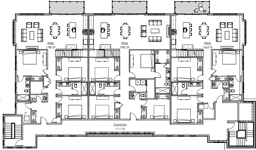
FOURTH FLOOR
