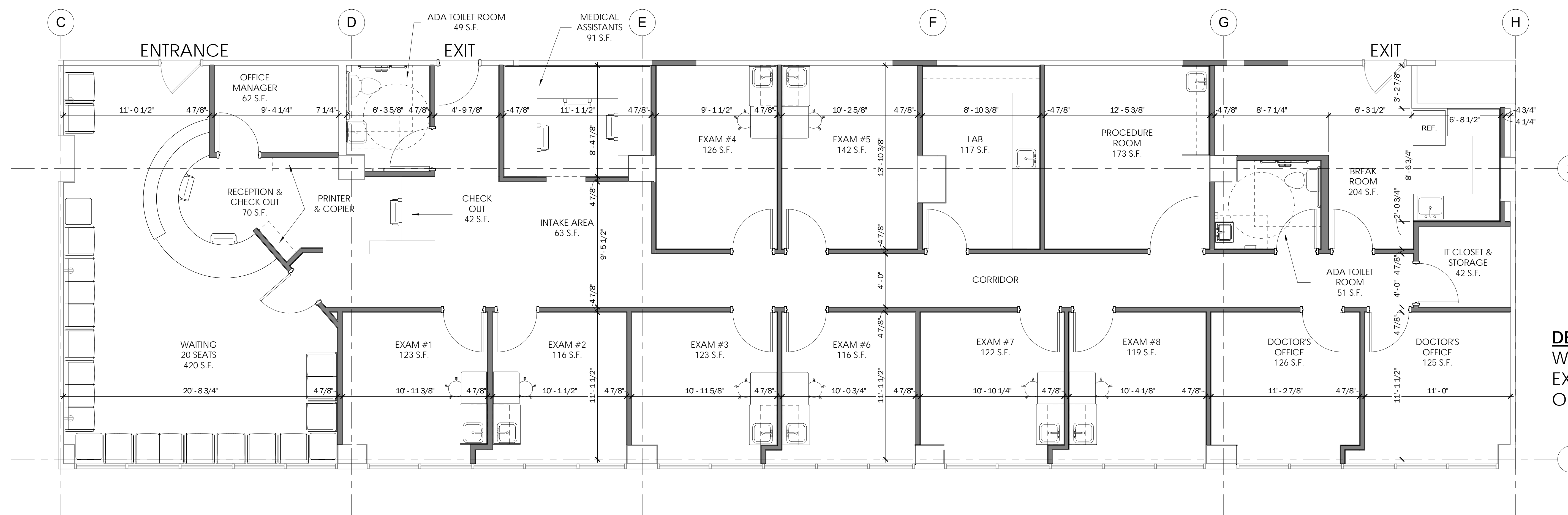
1 FIRST FLOOR PLAN - DESIGN OPTION 2 SK-106 1/4" = 1'-0"
