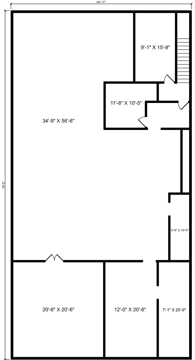
2ND FLOOR
