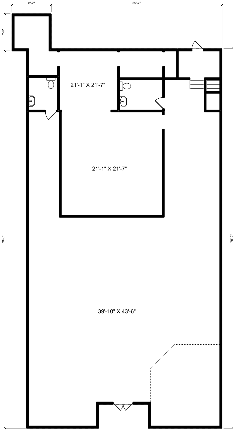
1ST FLOOR
