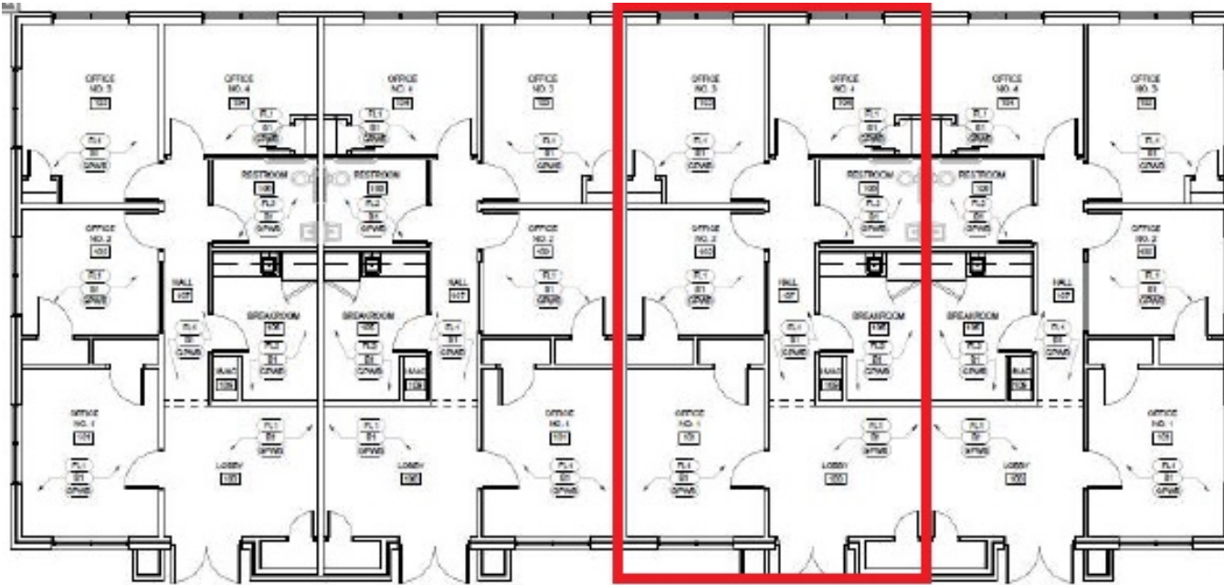
1 BUILDING A - FINISH FLOOR PLAN SCALE 3/8" = 1'-0"
