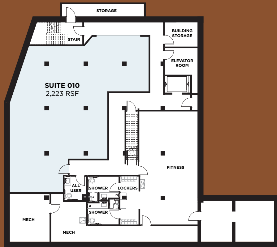
BASEMENT LEVEL
