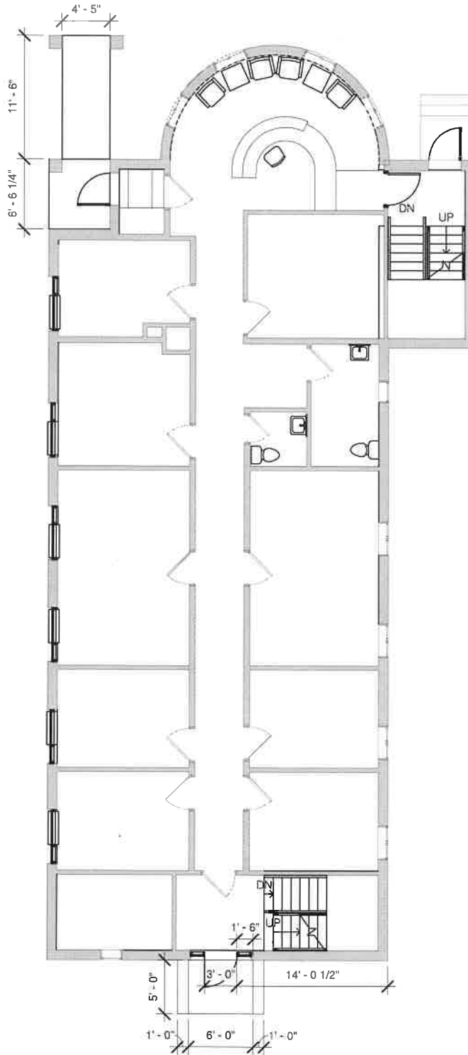
① FIRST FLOOR 1/8" = 1'-0"
