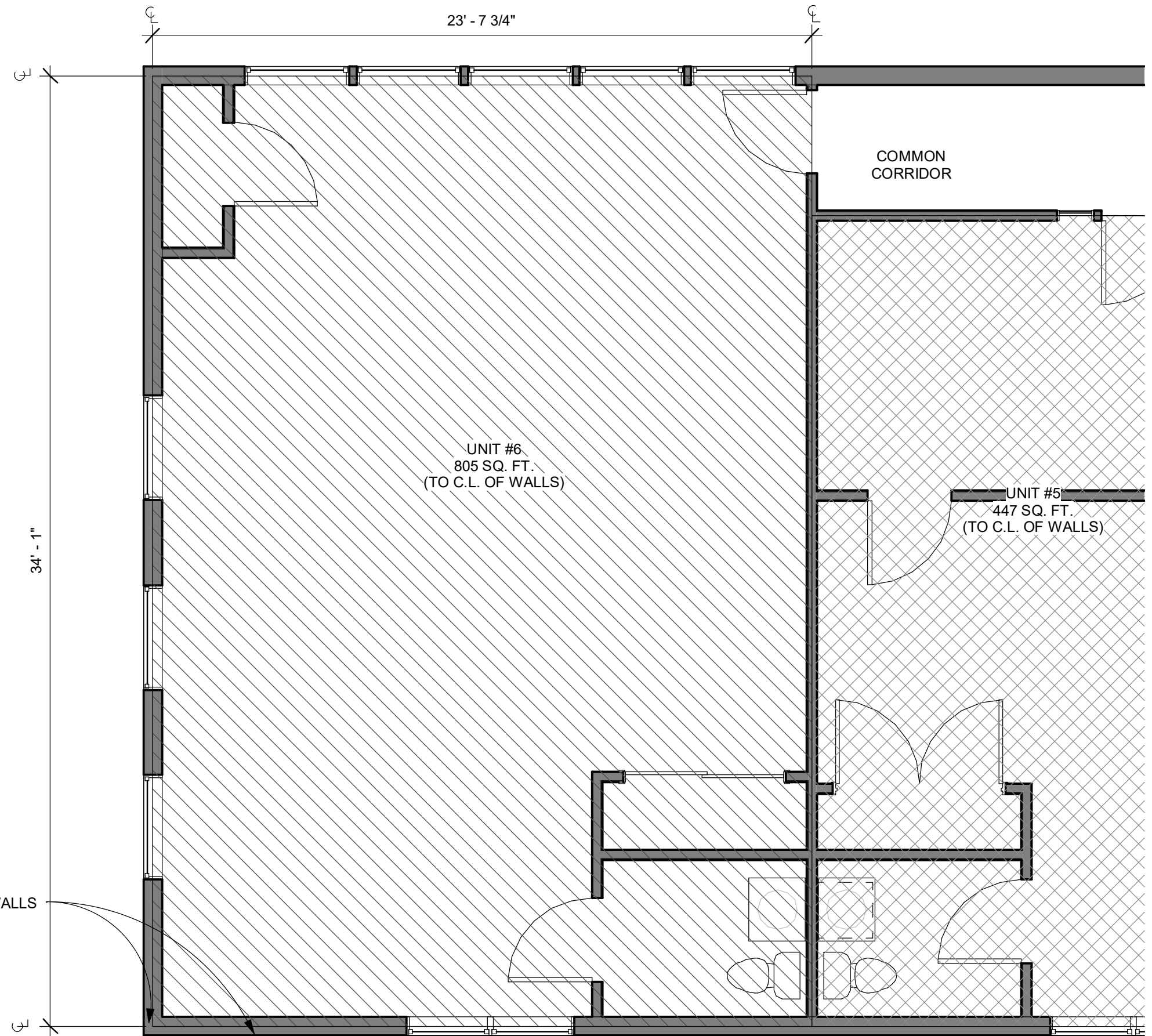
① UNIT 6 FLOOR PLAN 1/4" = 1'-0"
