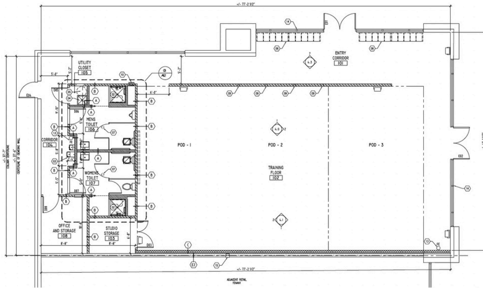
1 FLOOR PLAN
