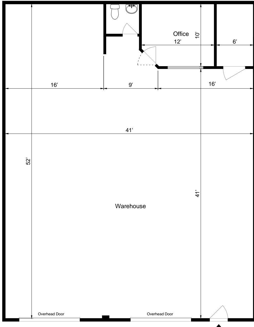
FLOOR PLAN
