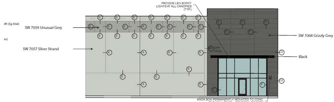
7 Exterior Elevation Detail Panel Joint and Reveal Keys 1/8"
