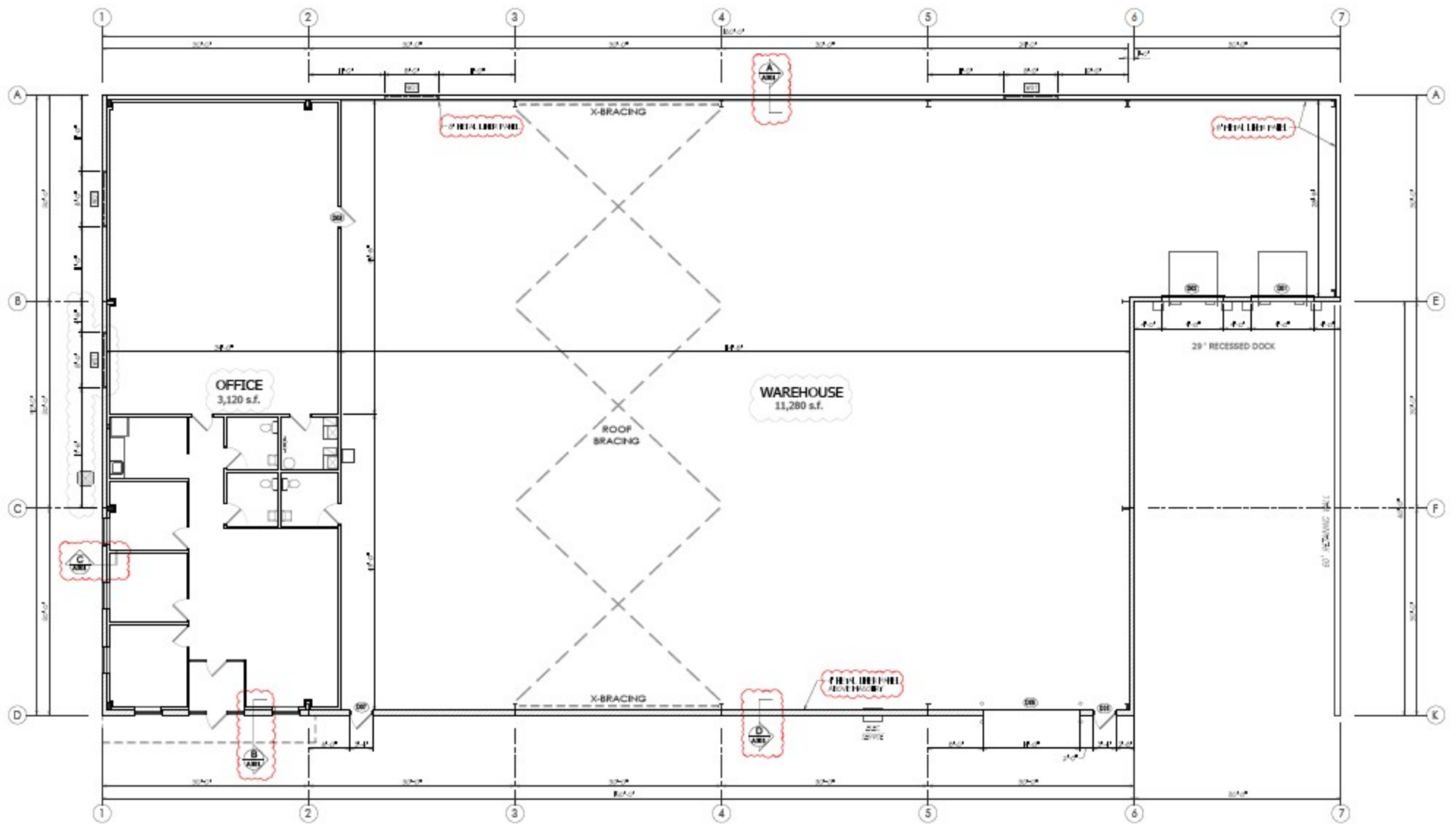
PROPOSED BUILDING PLAN SCALE: 1/8" = 1'-0"
