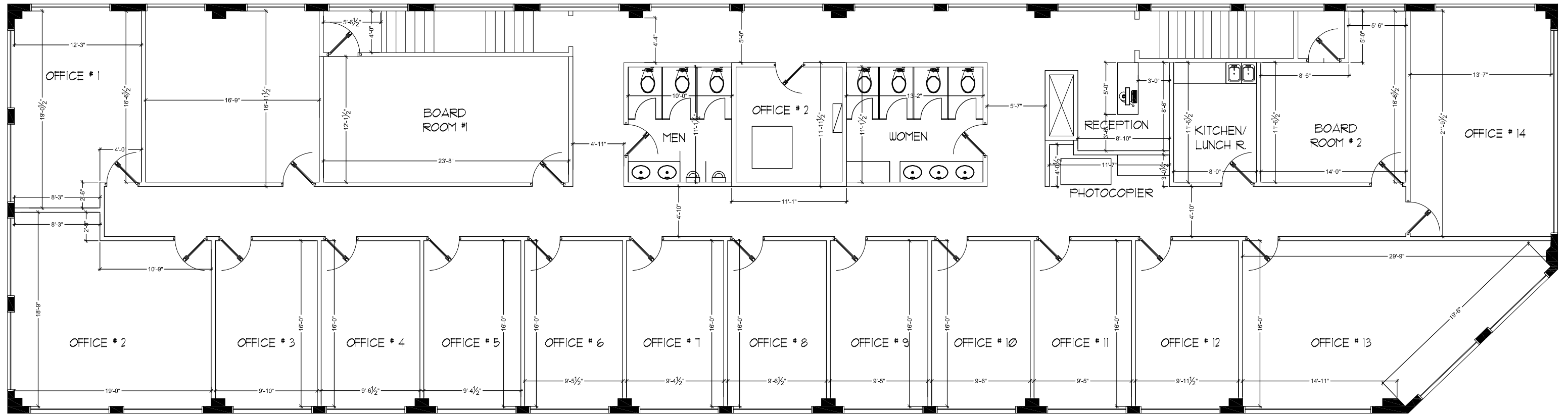
PROPOSED OFFICES FLOOR PLAN SCALE: N.T.S
