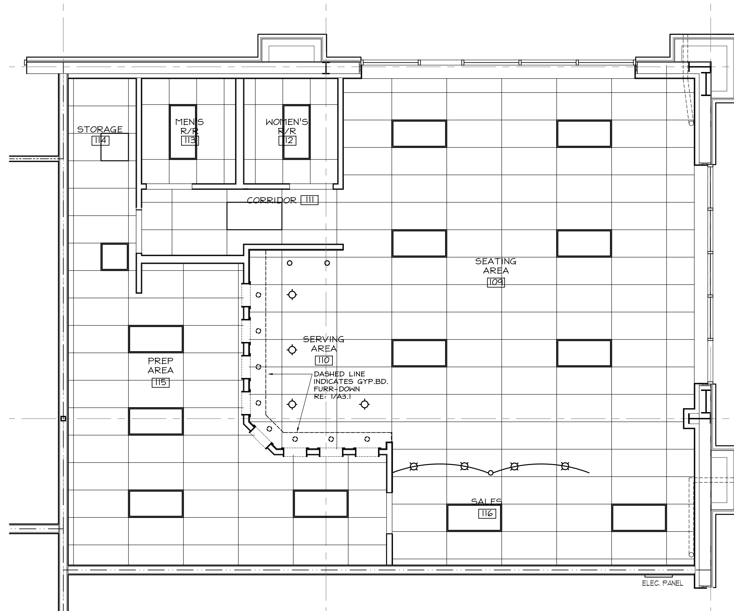
2 REFLECTED CEILING PLAN - ORANGE LEAF SCALE - 1/4" = 1'-0"
