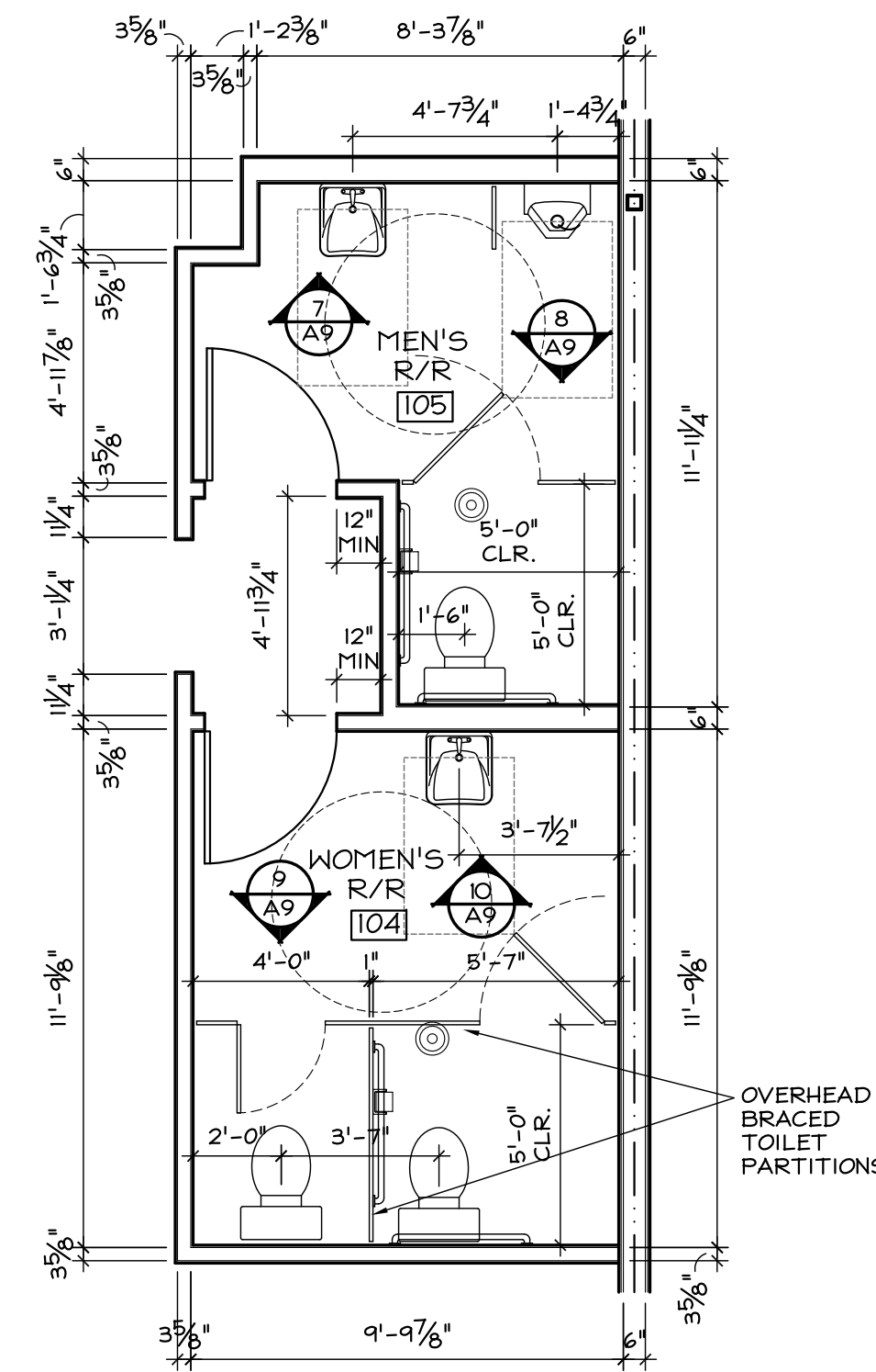
4 ENLARGED FLOOR PLAN RESTROOMS 104 & 105 SCALE - 1/4" = 1'-0"
