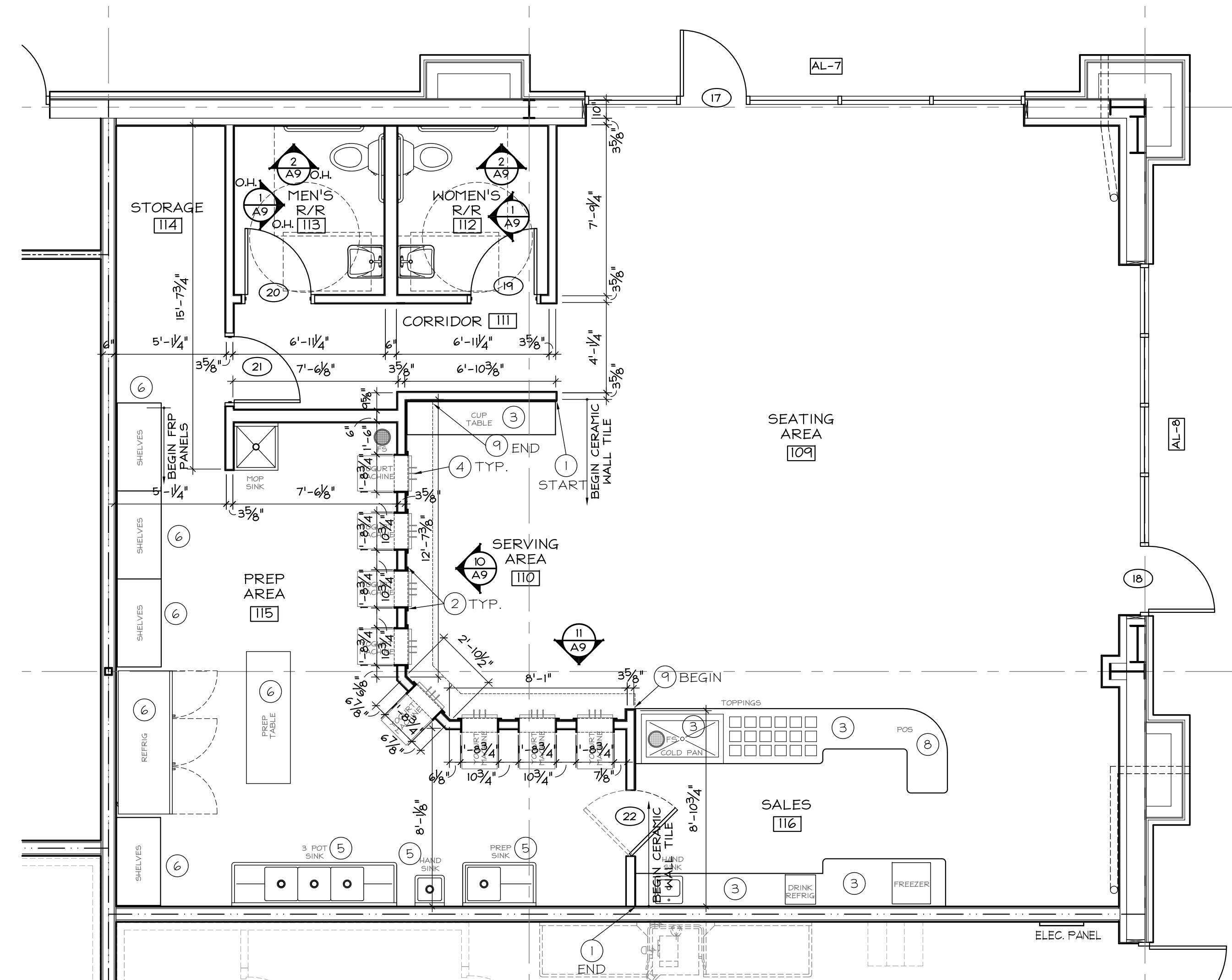
1 FLOOR PLAN - ORANGE LEAF SCALE - 1/4" = 1'-0"
