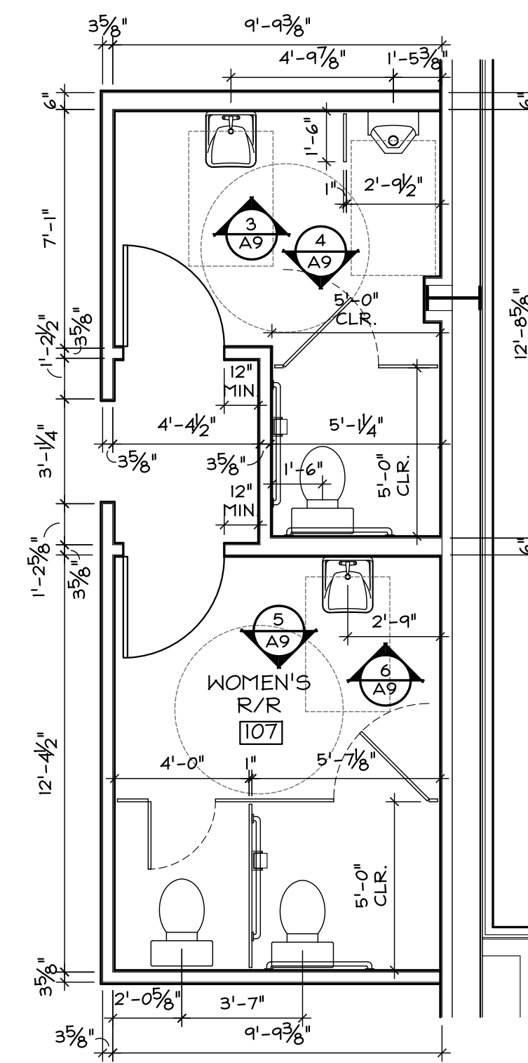
3 ENLARGED FLOOR PLAN RESTROOMS 107 & 108 SCALE - 1/4" = 1'-0"
