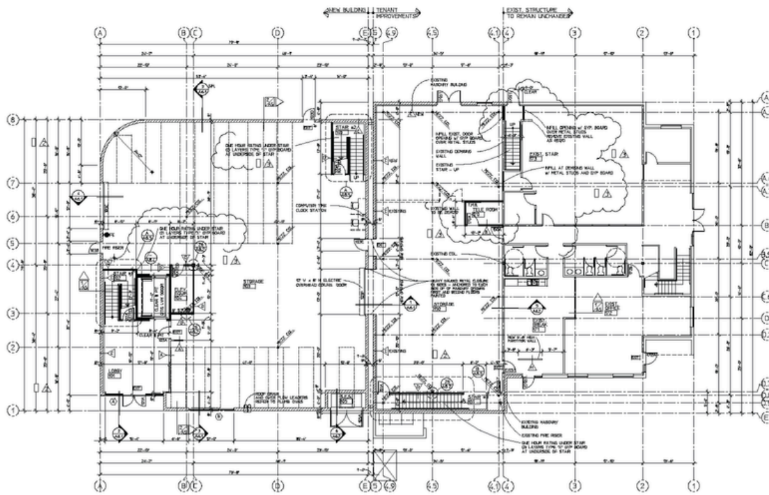
1st Floor
