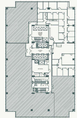
KEY PLAN
