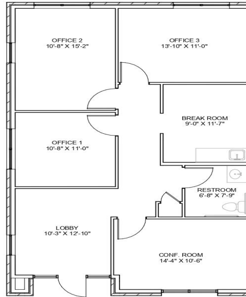
01 TYPICAL FLOOR PLAN - 1,187 SF SCALE: 1/8" = 1'-0"
