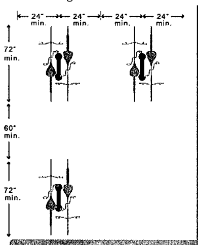
Bike Parking Dimensional Standards
