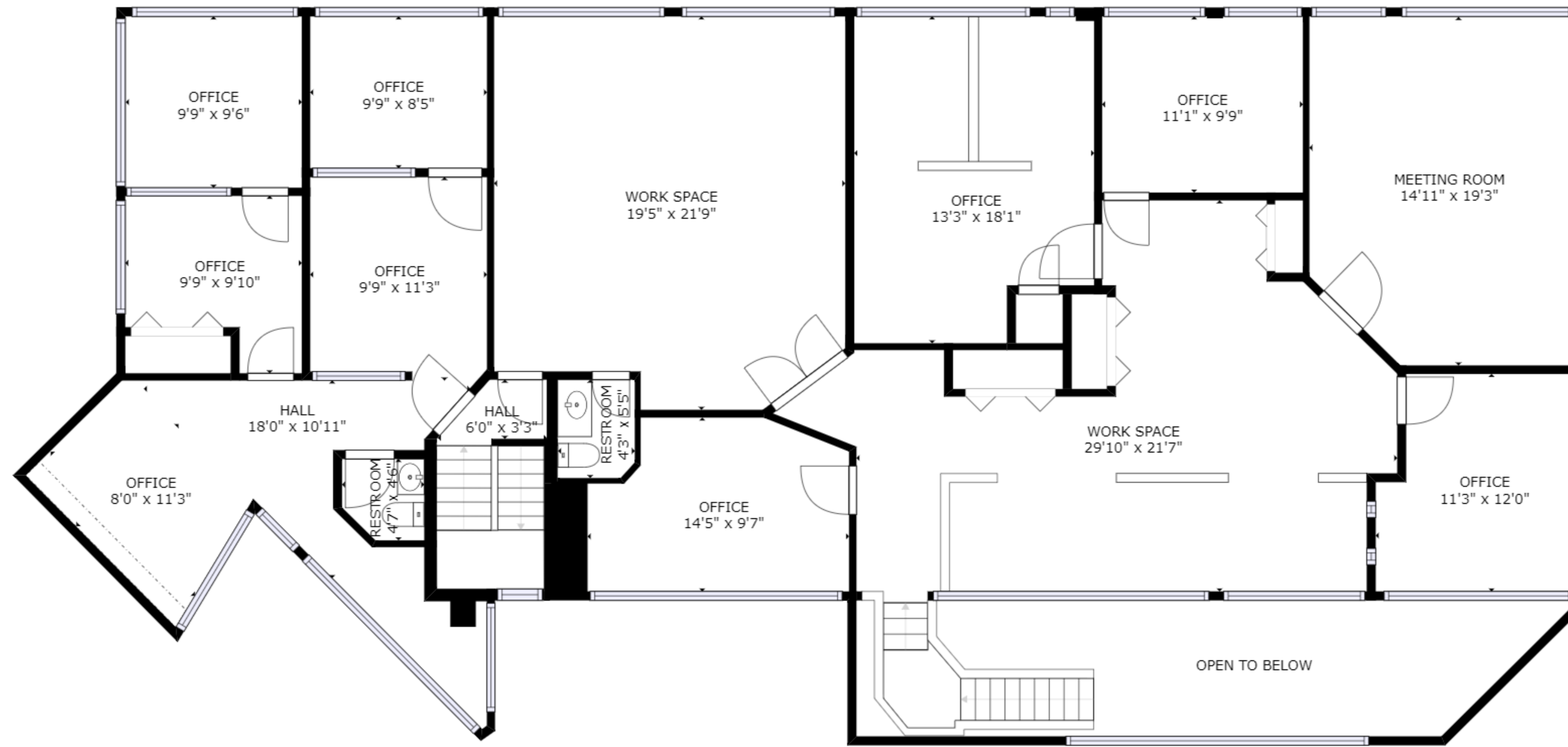
FLOOR 2
