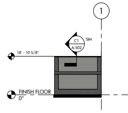
C2 RISER ROOM ELEVATION A-201 1/16" = 1'-0"
