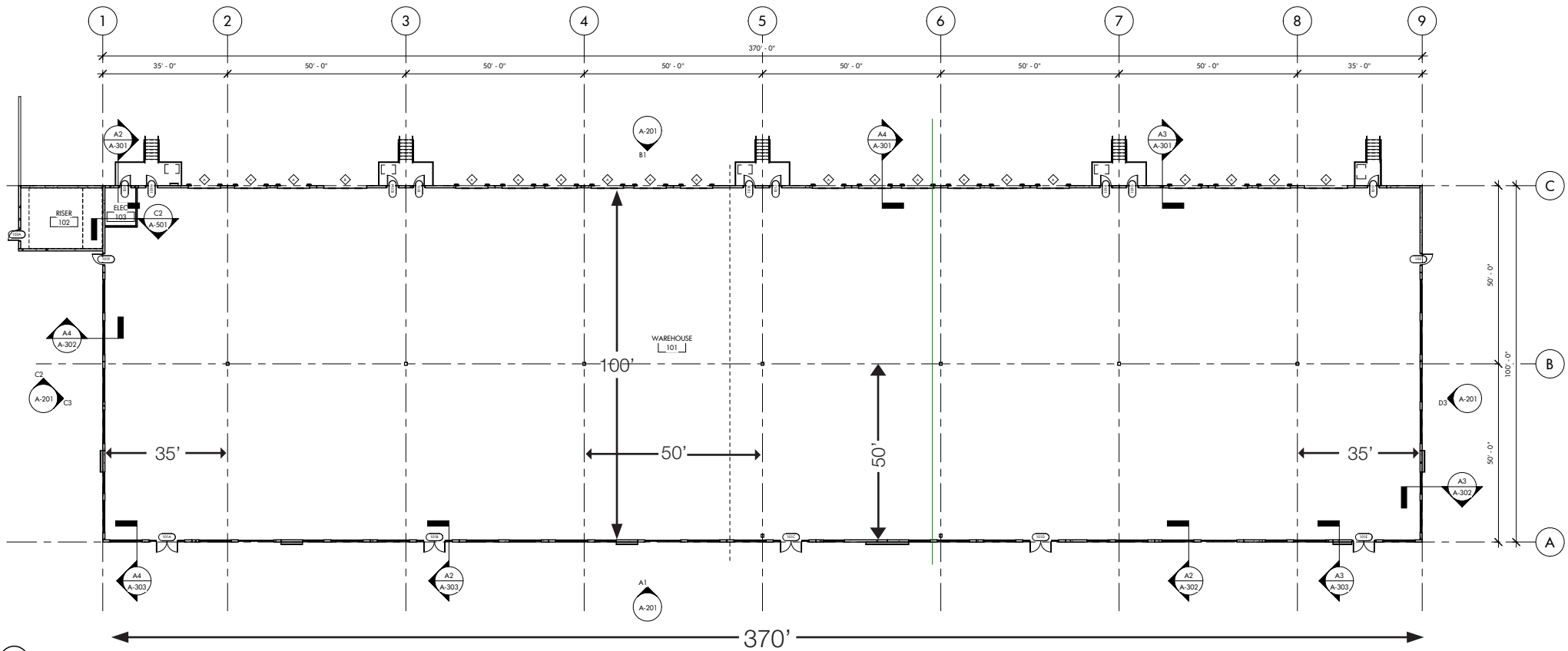
A1 FIRST FLOOR PLAN
