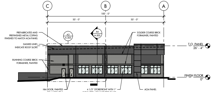
C3 PLAN WEST ELEVATION A-201 1/16" = 1'-0"
