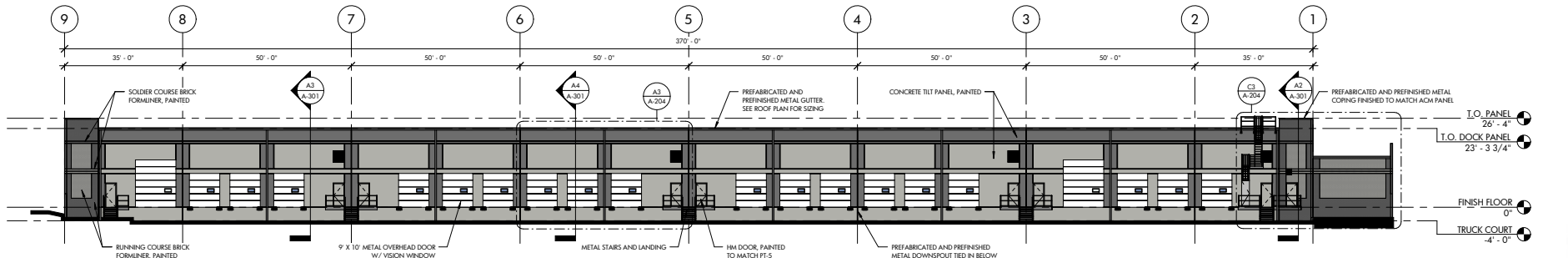
B1 PLAN NORTH ELEVATION A-201 1/16" = 1'-0"
