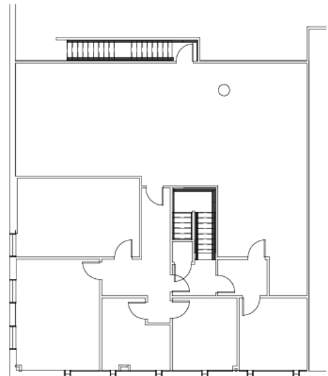
MEZZANINE LEVEL
