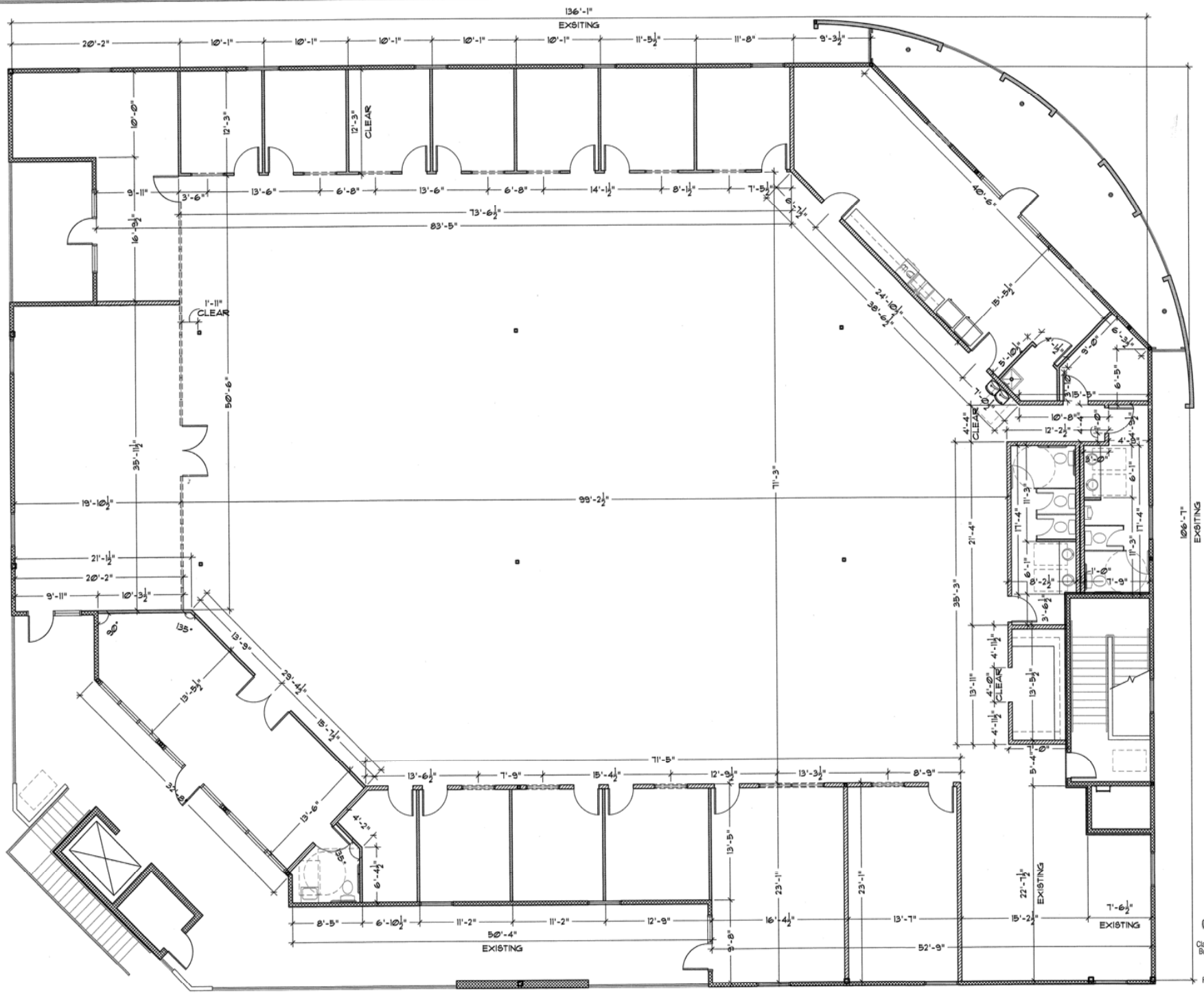
DIMENSION PLAN SCALE 3/16"=1'-0"
