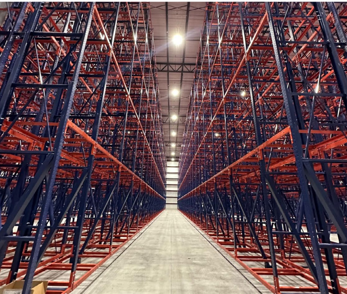
PROPOSED RACK
