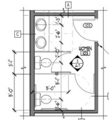
4 ENLARGED FLOOR PLAN SCALE: 1/4" = 1'-0"
