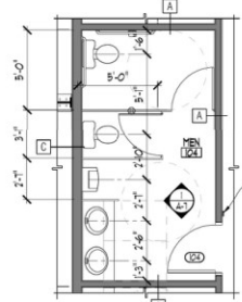
3 ENLARGED FLOOR PLAN SCALE: 1/4" = 1'-0"
