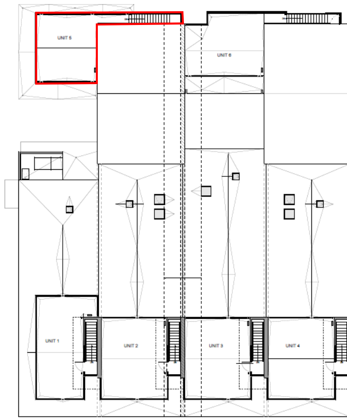
ROOF DECK PLAN 464 W OCEAN FRONT WALK
