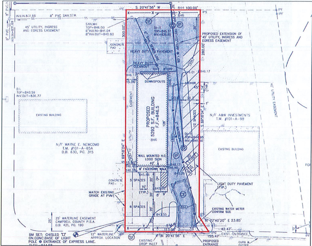
SITE PLAN
