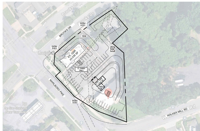
CONCEPTUAL LAYOUT 04
