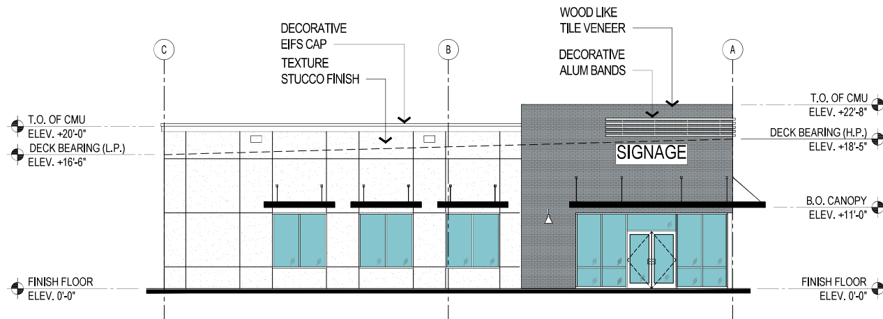
SIDE (SOUTH) ELEVATION
