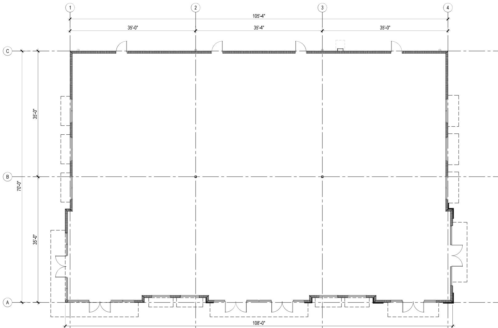
FLOOR PLAN 7,396 S.F.
