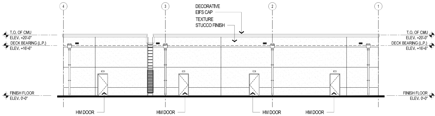
REAR (WEST) ELEVATION
