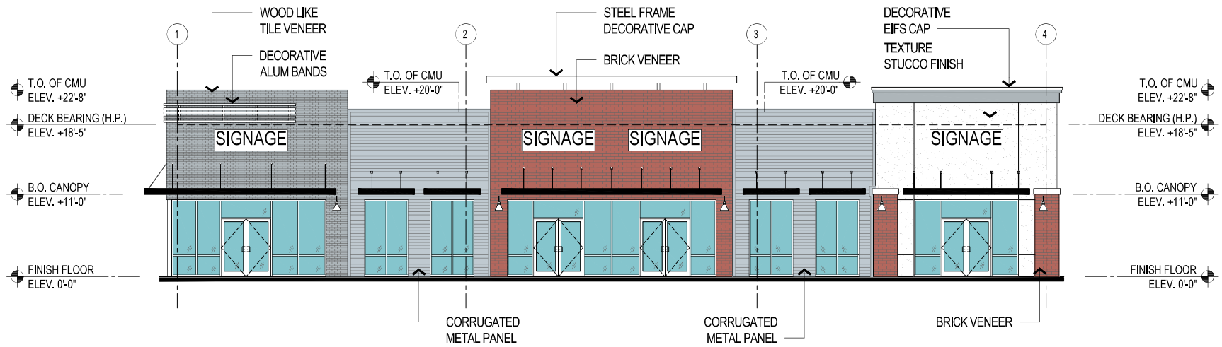
FRONT (EAST) ELEVATION
