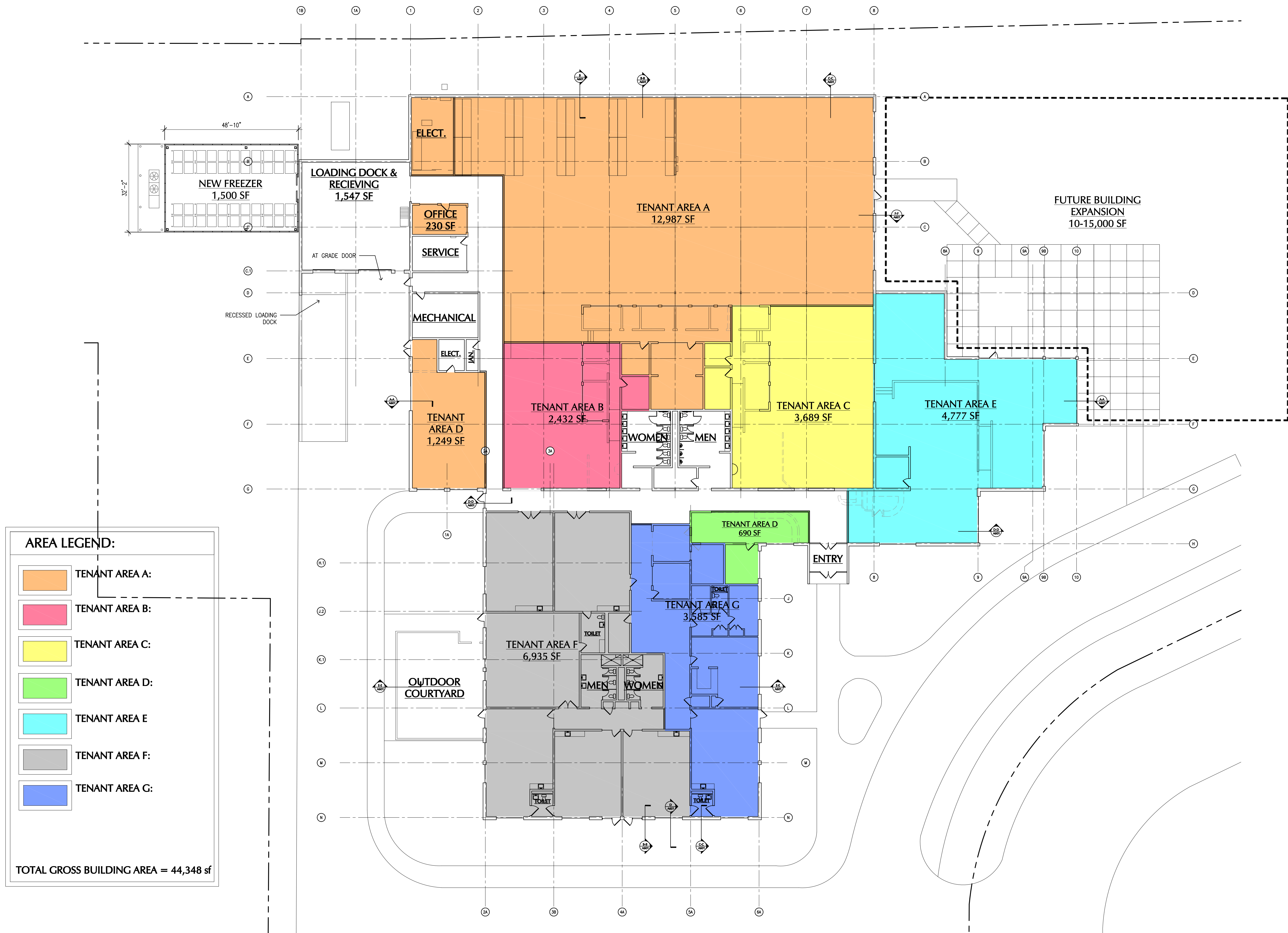
1 OVERALL FLOOR PLAN ID101 SCALE: 1/16" = 1'-0"
