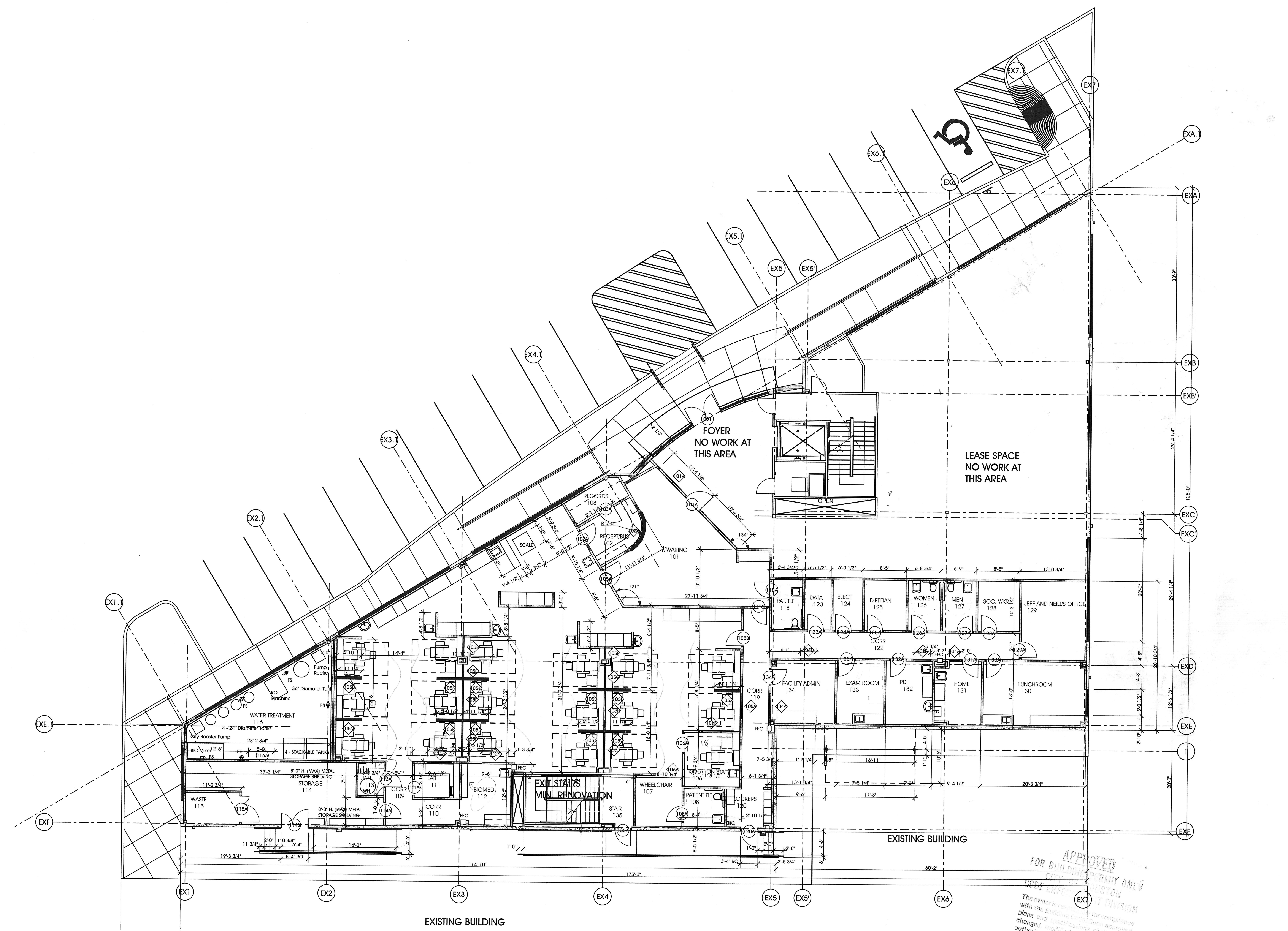
1 FIRST FLOOR DIMENSION PLAN SCALE: 1/8" = 1'-0"
