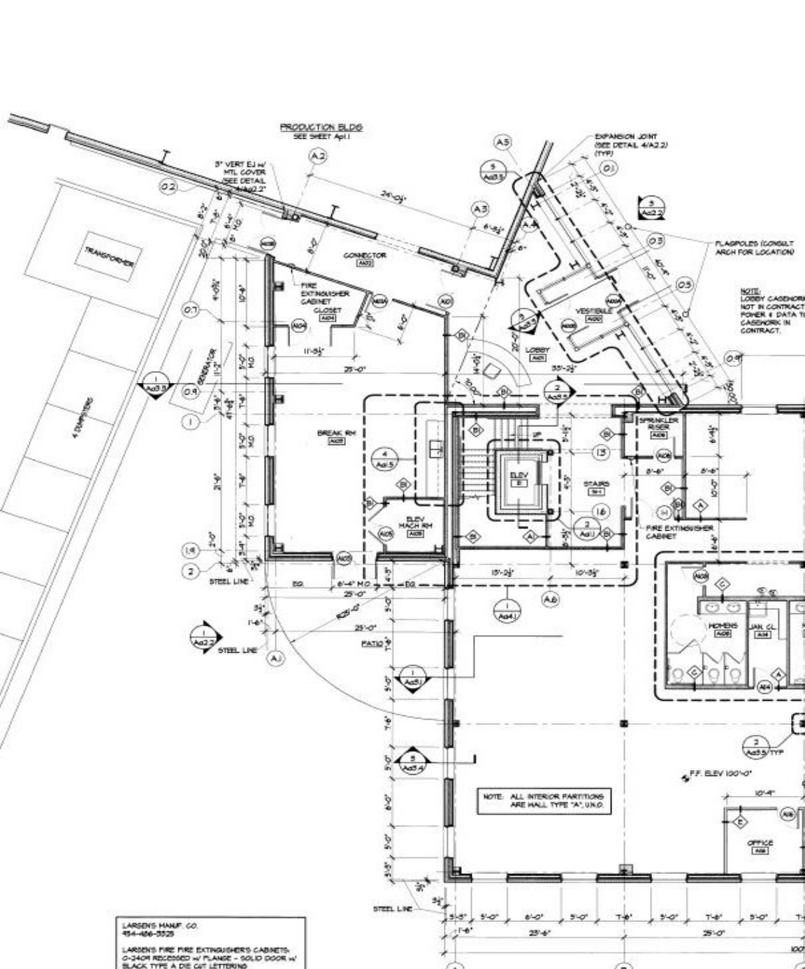
1 FIRST FLOOR PLAN - ADMIN. BLDG. SCALE: 1/8" = 1'-0"
