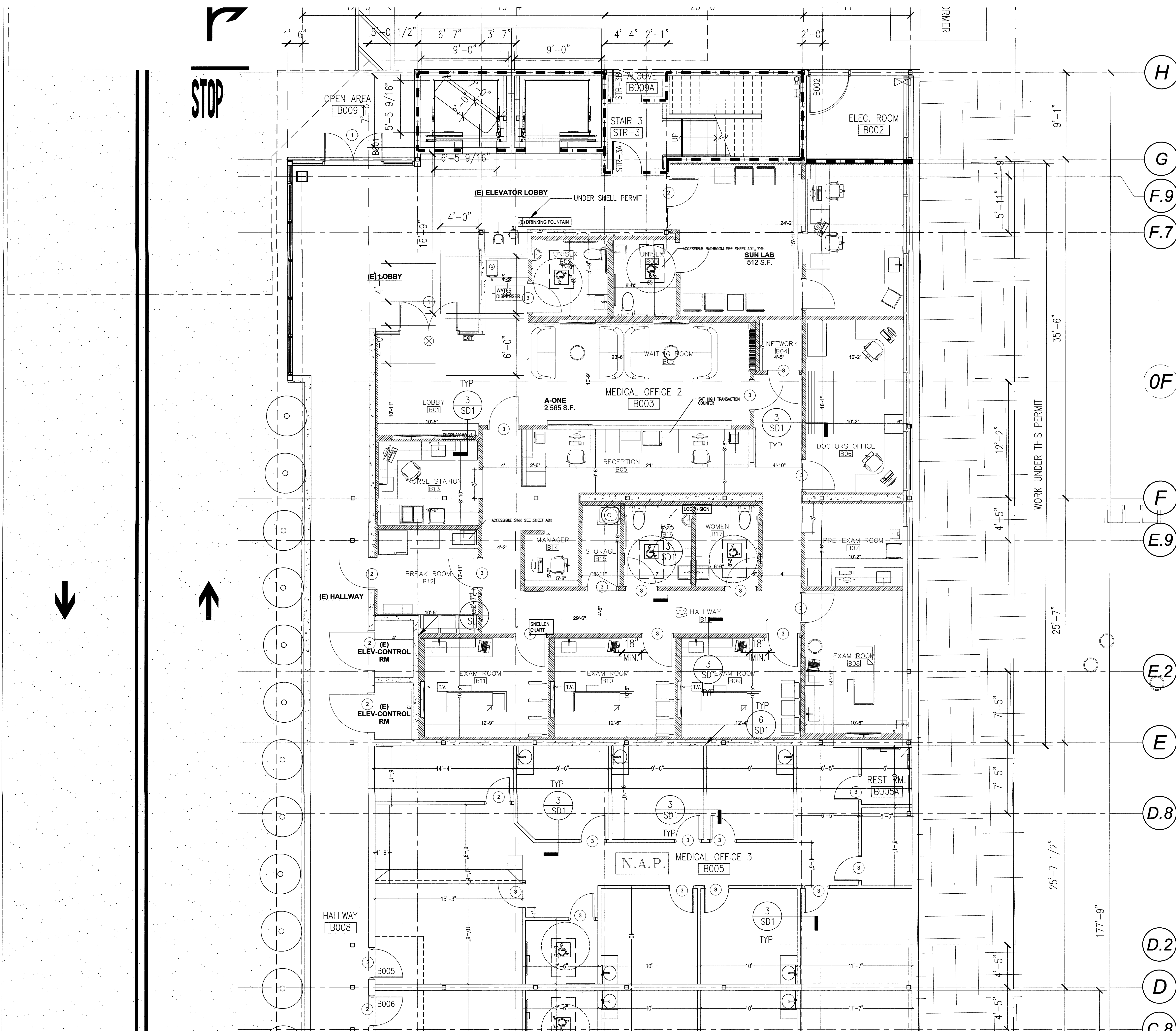
SUITES B003 & B004 TI FLOOR PLAN
