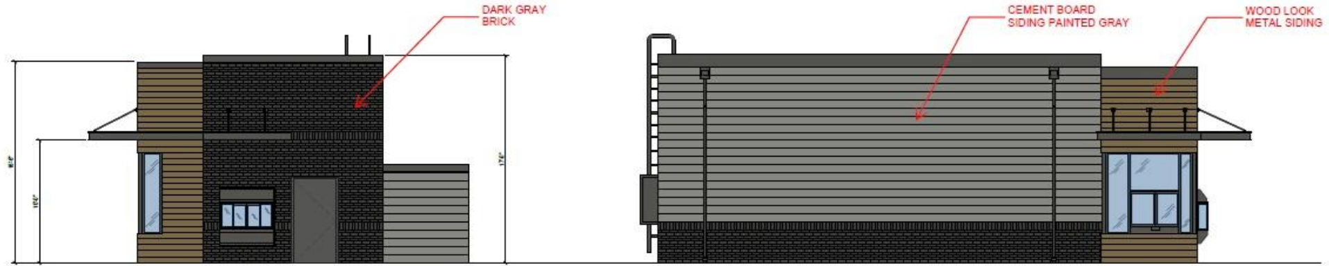
1 PRELIMINARY WEST (FRONT) ELEVATION A3.1 1/4" = 1'-0"
