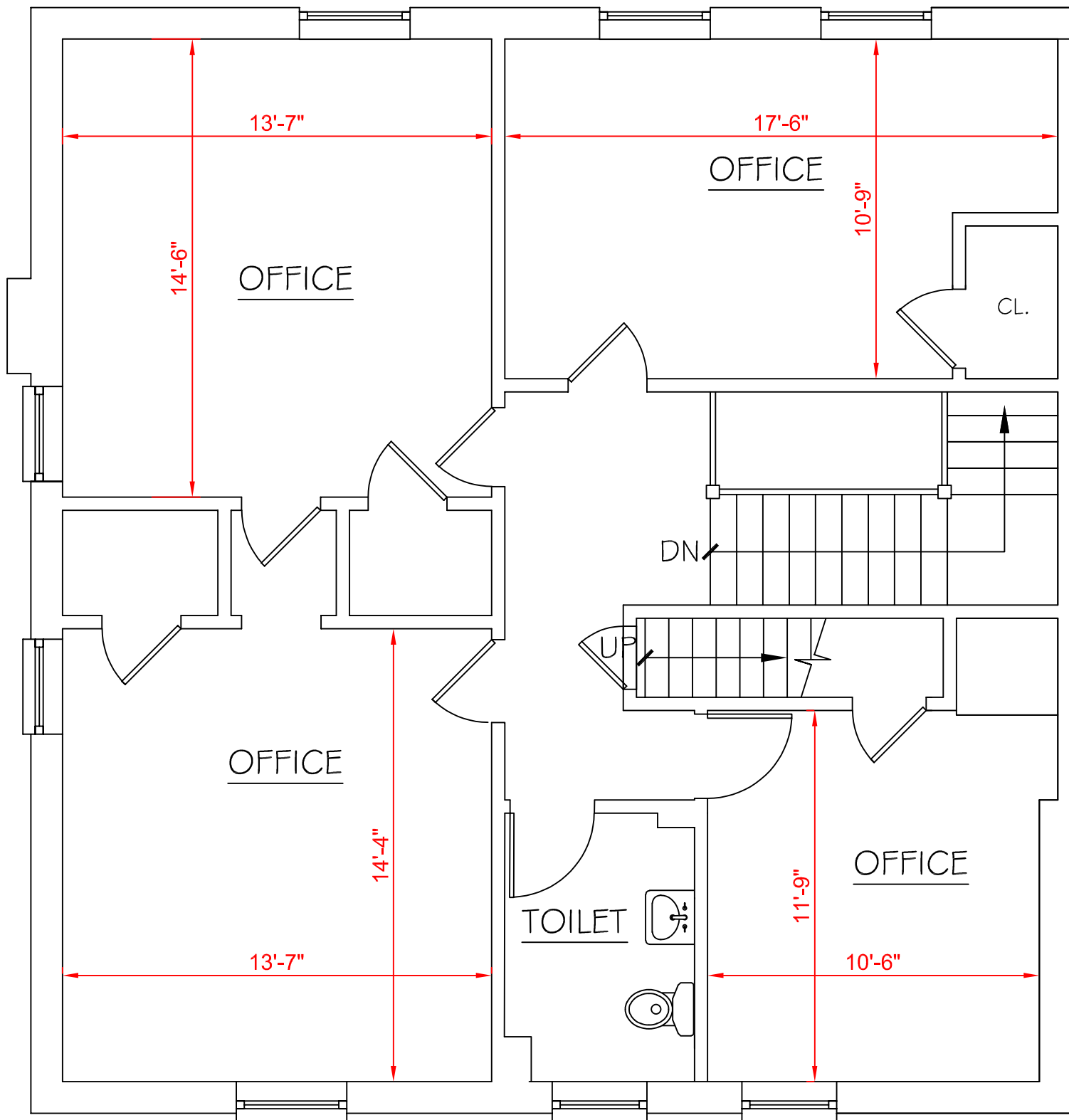
Quarters M-6 2nd Floor
