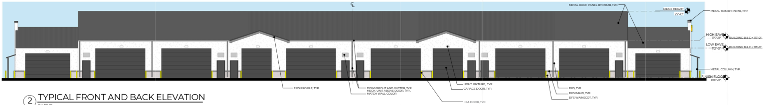
2 TYPICAL FRONT AND BACK ELEVATION 1" = 32'-0"
