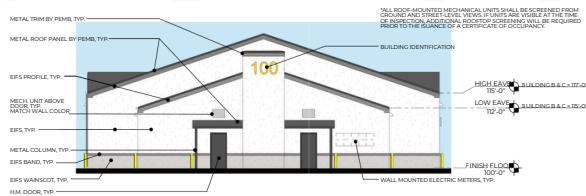
3 TYPICAL SIDE ELEVATION 1" = 32'-0"
