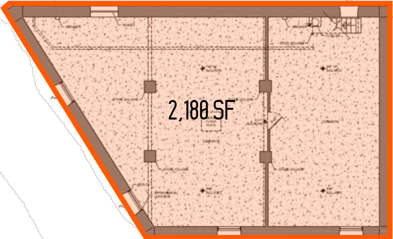
Basement
